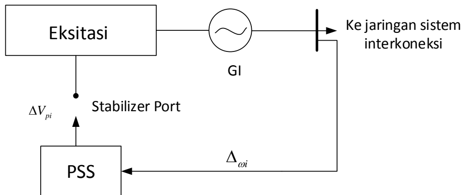
Figure 3. A PSS System in the i-Generator
