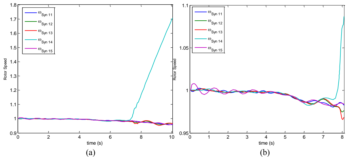
Figure 7. Graph of Rotor angle velocity for generator 11-15. (a) Without PSS, (b) With PSS
