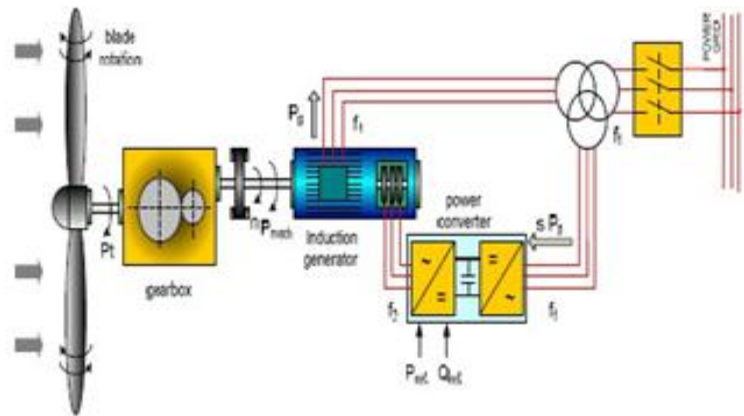
Figure 2. System Double Fed Induction Generator (DFIG)
