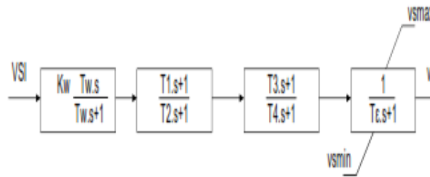
Figure 4. Second type of PSS
